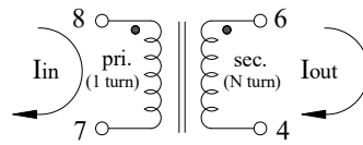
CT050A Series SCHEMATIC
