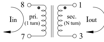
CT050 Series SCHEMATIC
